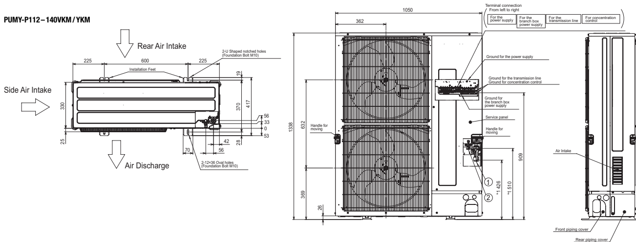
PUMY-SP112-140VKM/YKM
